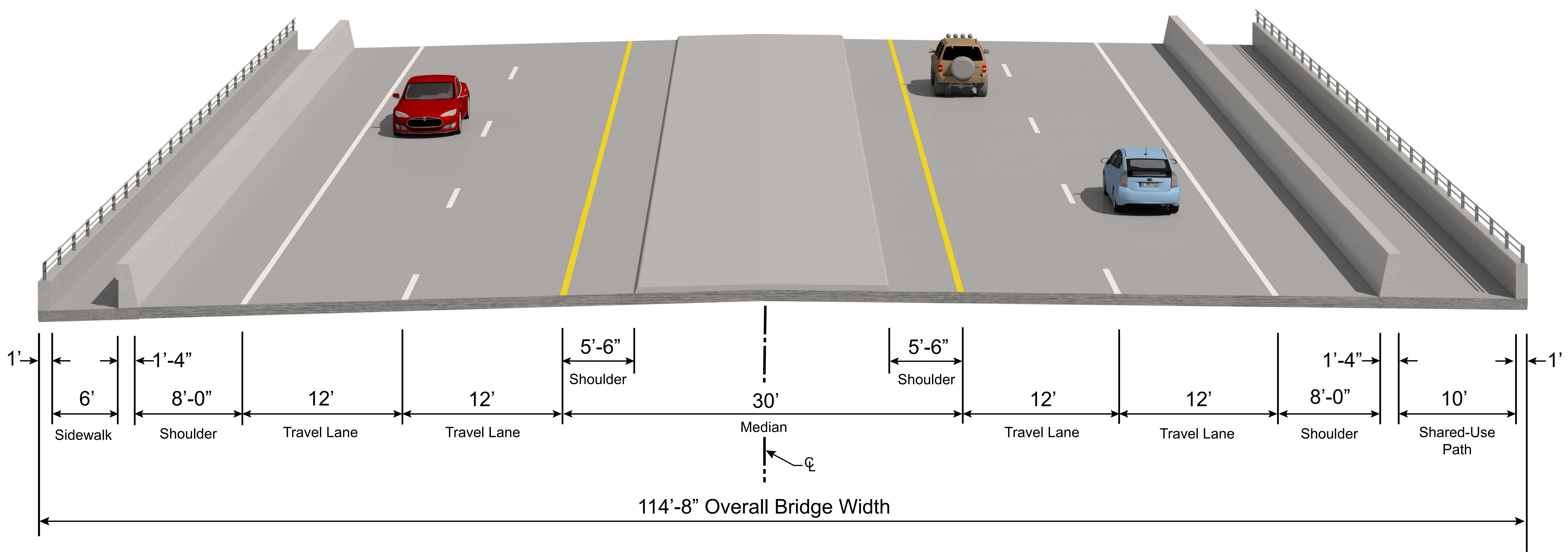
PROPOSED BRIDGE TYPICAL - OVER SOTTILE CANAL
