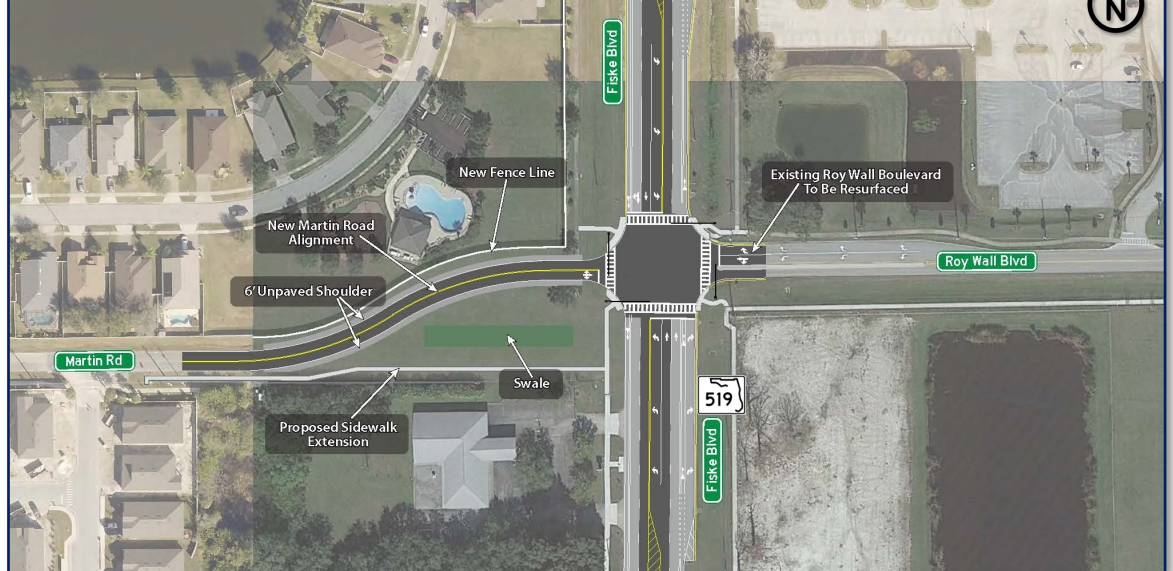
Rendering: Aerial View of Realigned Intersection
