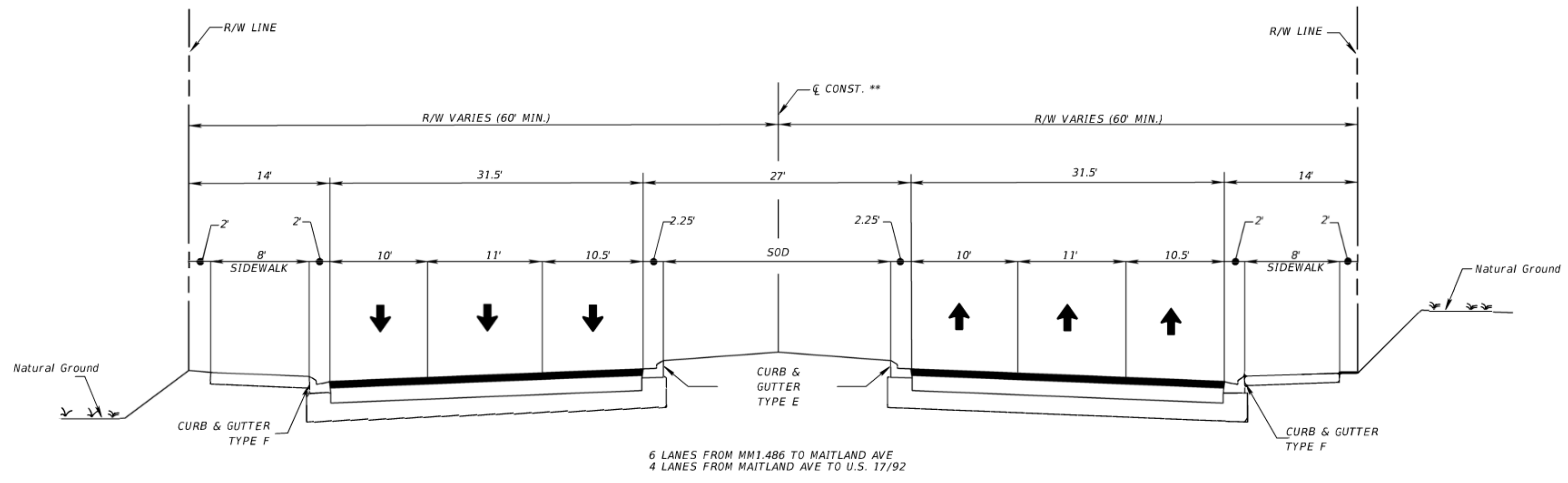
TYPICAL SECTION S.R. 414 (MAITLAND BOULEVARD) LAKE FAITH DRIVE TO THE END OF THE U.S. 17-92 RAMPS
