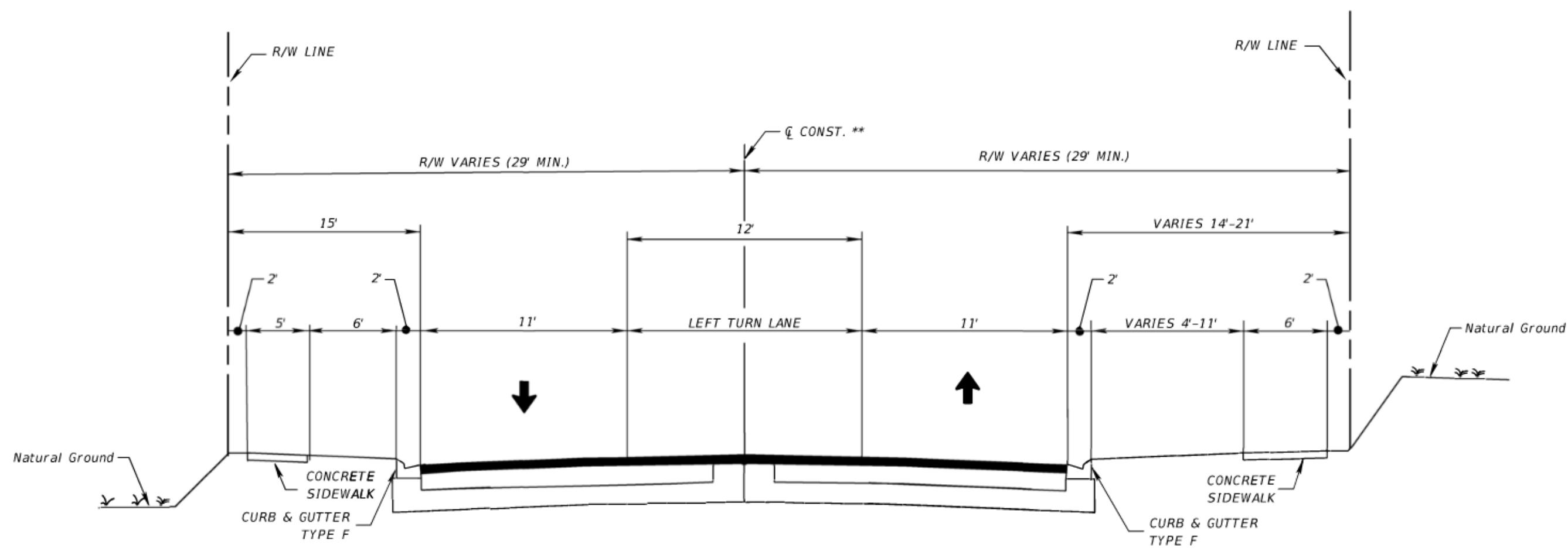
TYPICAL SECTION MAITLAND AVENUE U.S. 17-92 TO HORATIO AVENUE
