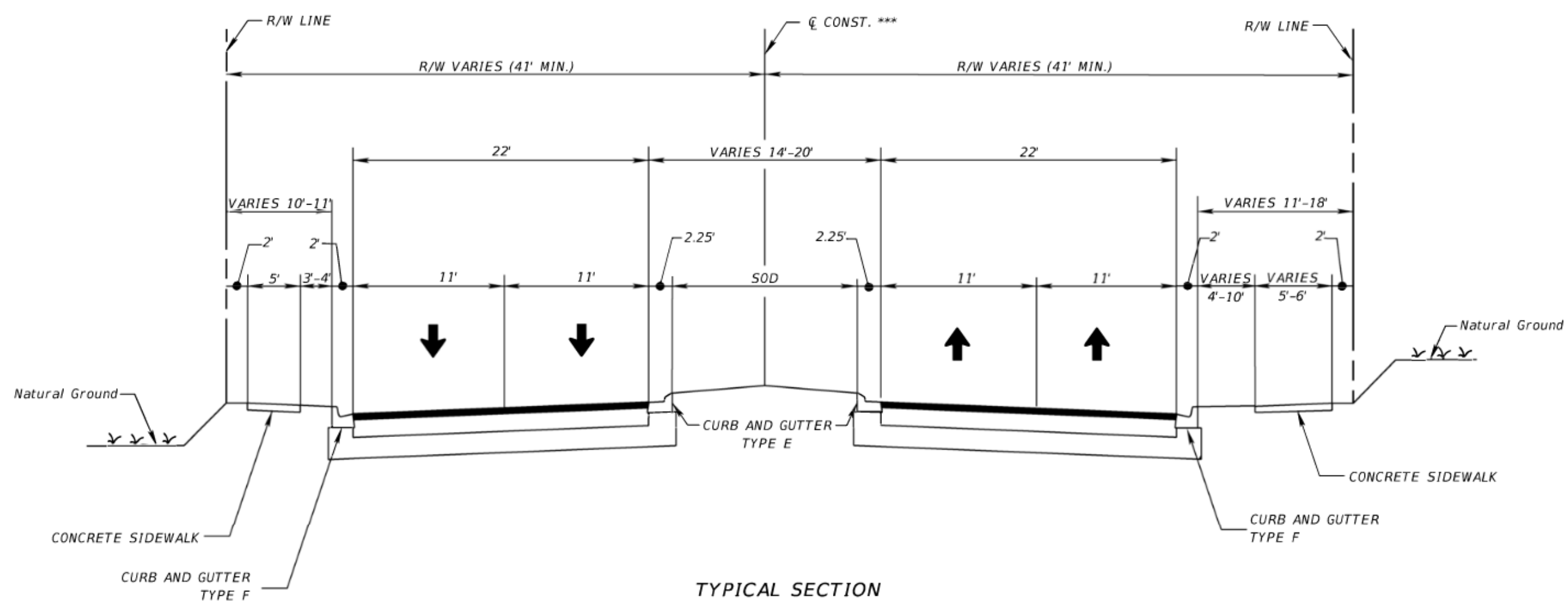
TYPICAL SECTION MAITLAND AVENUE HORATIO AVENUE TO S.R. 414 (MATILAND BLVD)
