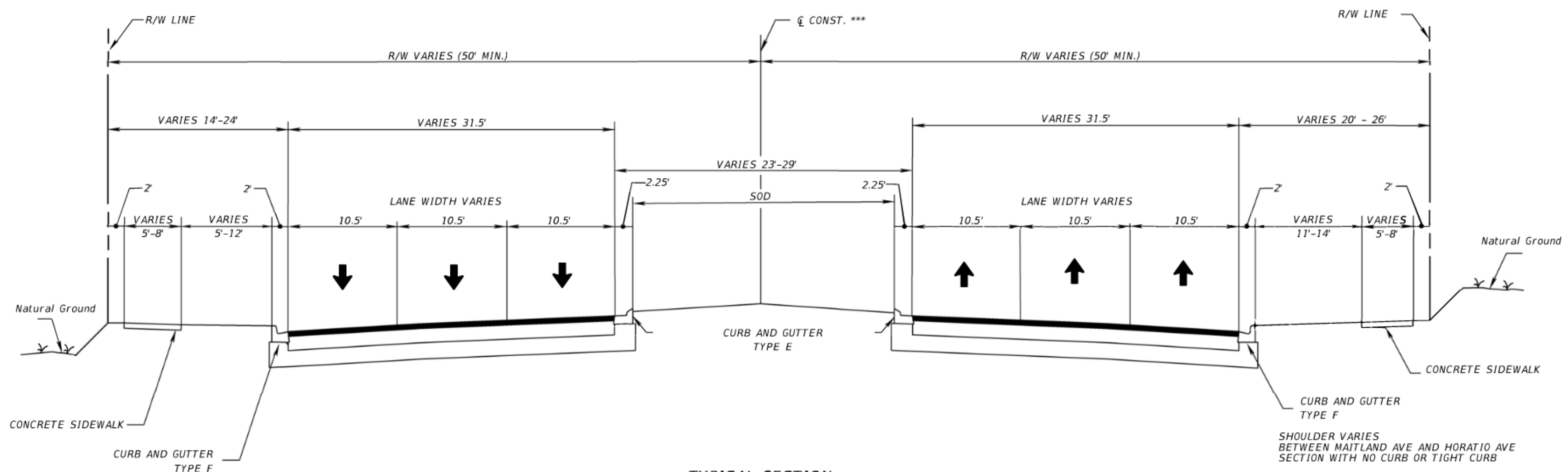
TYPICAL SECTION U.S. 17-92 (ORLANDO AVENUE) 560FT SOUTH OF MAITLAND AVENUE TO THE SEMINOLE COUNTY LINE
