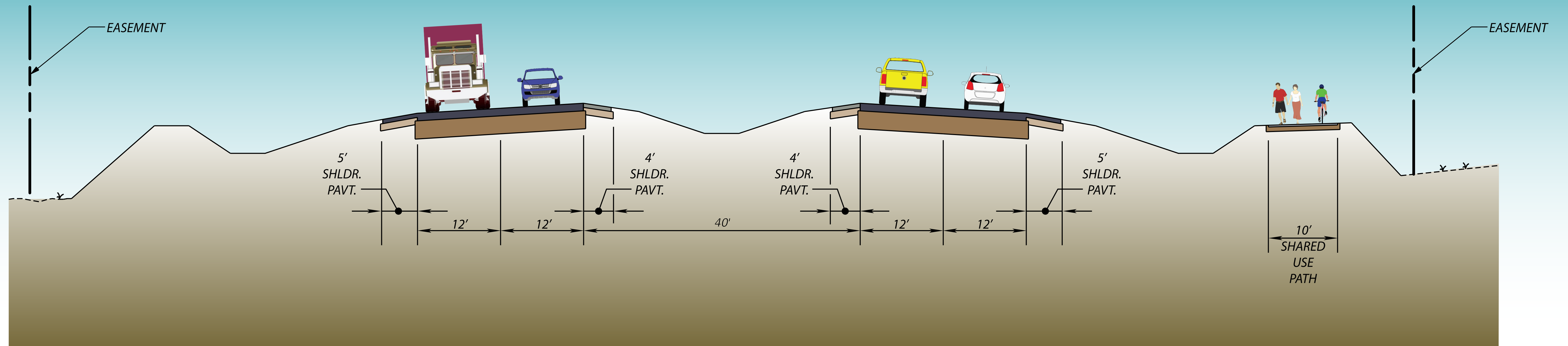
TYPICAL SECTION No. 2 FROM BURWELL TO COUNTY LINE
