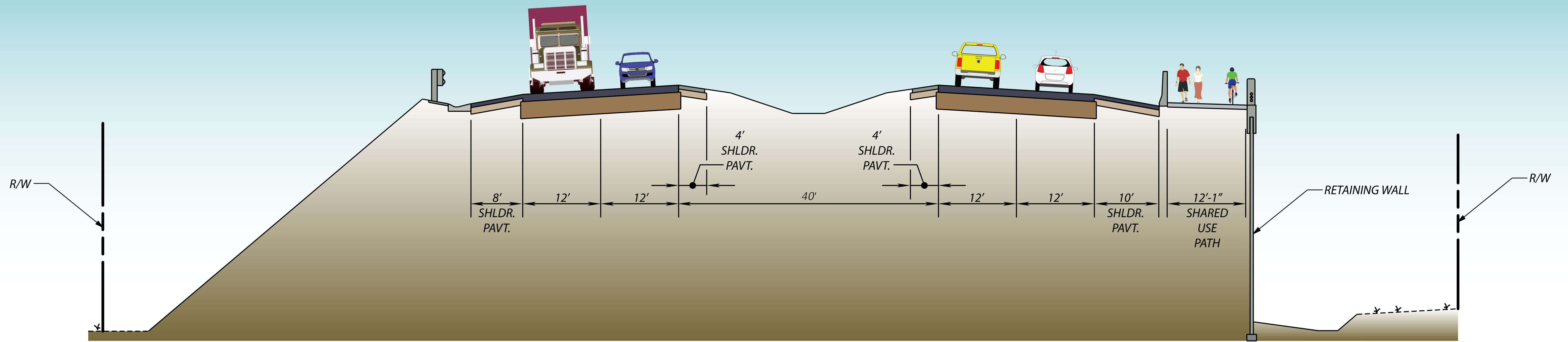
TYPICAL SECTION No. 1 FROM WEST FLORIDA AGGREGATE TO BURWELL ROAD
